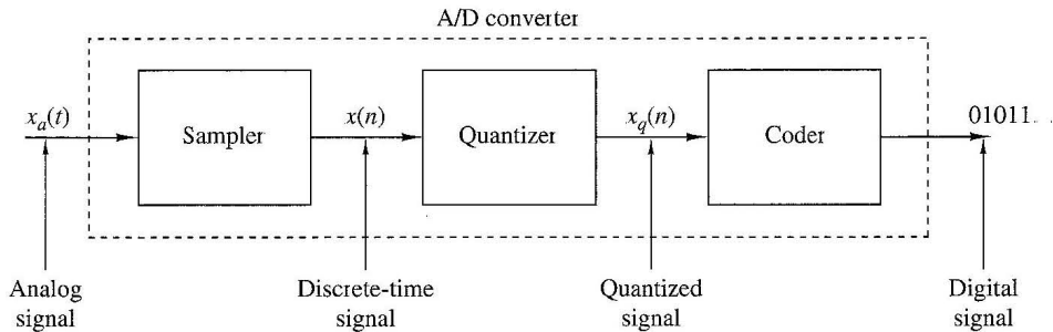
Figure 1.4.1 Basic parts of an analog-to-digital (A/D) converter.
